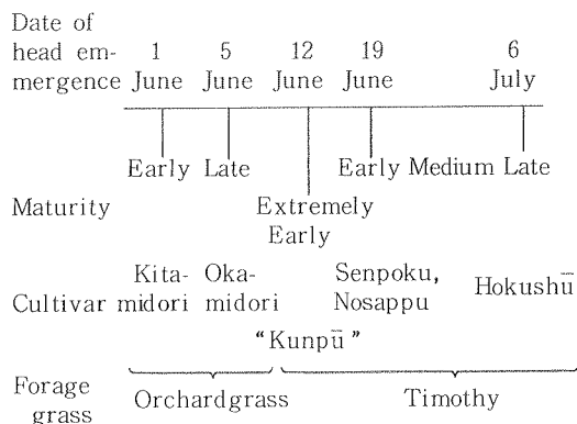
Fig. 1 Array of date of head emergence in two forage grasses and their cultivars observed at Kitami Agric. Exp. Stn, Kunneppu.
