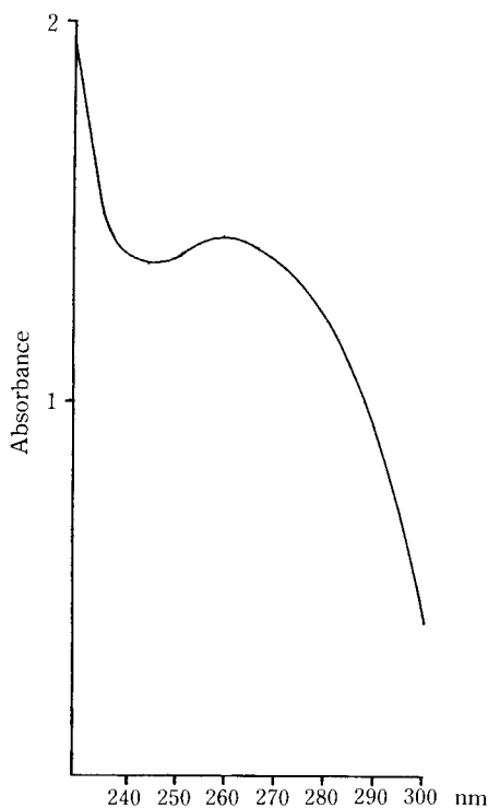
Fig. 26. UV absorption spectrum of purified SDV.
