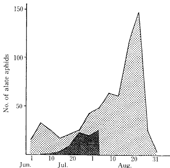
Fig. 20. The number of alate aphids caught on cylindrical yellow sticky traps at 1981~1982. 1981: 1982:
