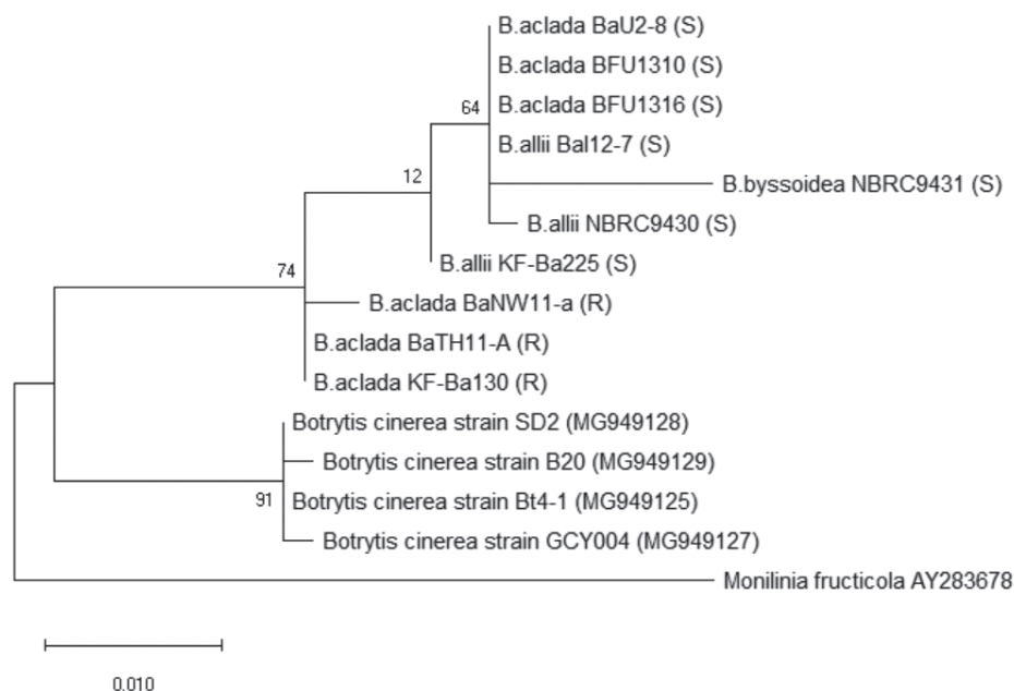
Fig. 7. A phylogenetic tree based on \beta -tubulin partial sequence of Hokkaido isolates of gray-mold neck of onion and DDBJ database.
