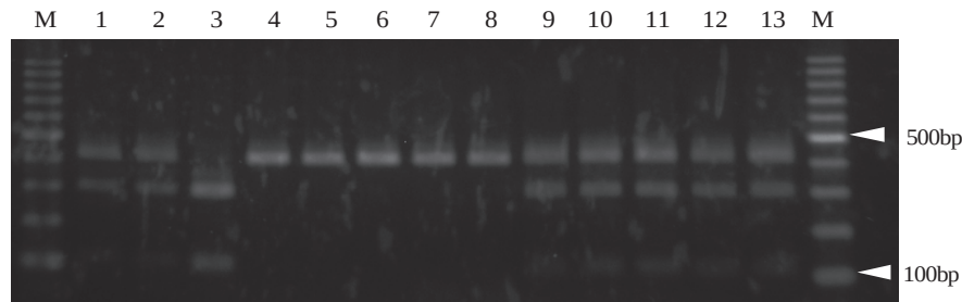
Fig. 3. ApoI restriction digestion of the PCR product of Botrytis spp. from onion bulbs.
