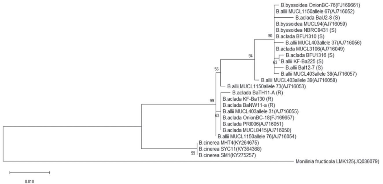
Fig. 8. A phylogenetic tree based on HSP60 partial sequence of Hokkaido isolates of gray-mold neck of onion and DDBJ database. NBRC 9430 and NBRC 9431 were supplied as B. allii and B. byssoidea from NITE, respectively. Monilinia fructicola was used as an outgroup.
