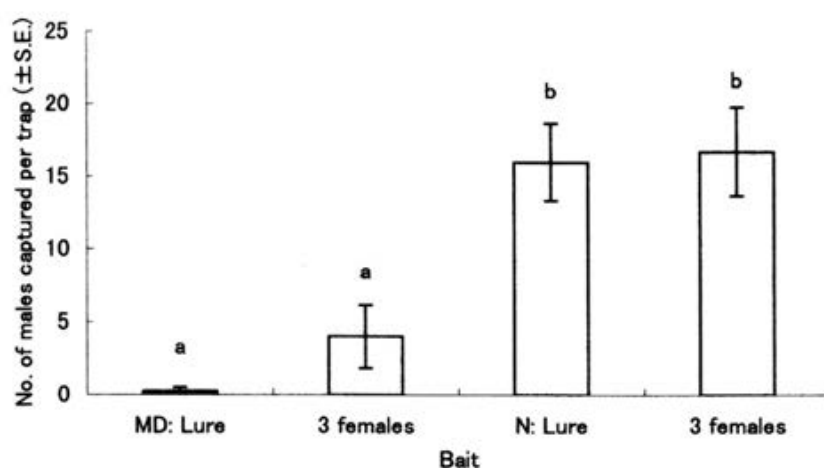
Figure 4-6. Effect of trapping disruption of Trigonotylus caelestialium males attracting to the 3-component pheromone trap by high concentration treatments of the sex pheromone components in small-scale field experiment (test 5: 15-29 Aug. 2003). MD: field treated with the dispenser loaded with 300 mg of the 3-component sex pheromone; N, untreated field. The means followed by the same letter are not different at the 5 % level by Tukey's test.
