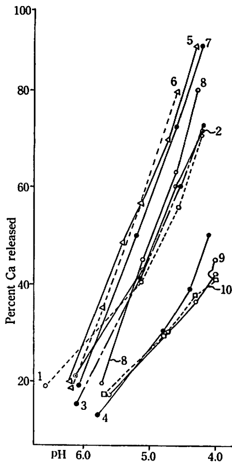
Fig. 6 Effect of addition of normal acetic acid solution on pH value of Ca-soil and Ca released
