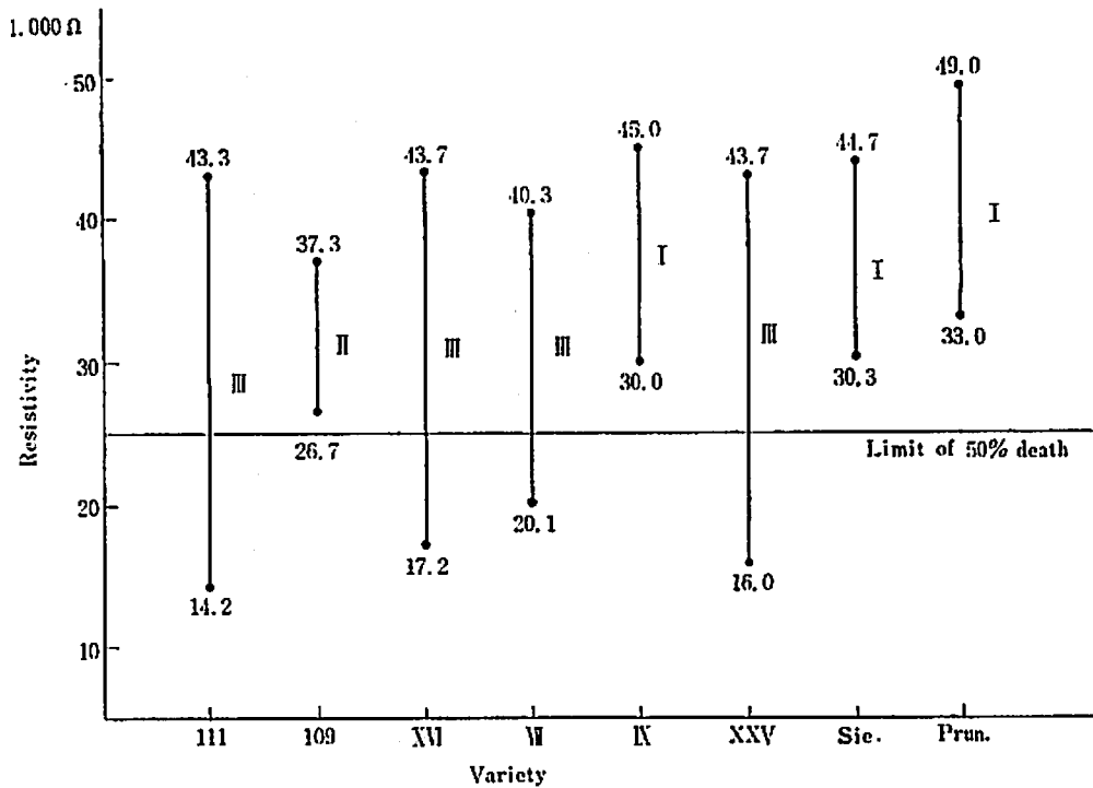
Fig. 3 Frost hardness of shoots in mid-autumn (Oct. 12) (See Tab. 3)
