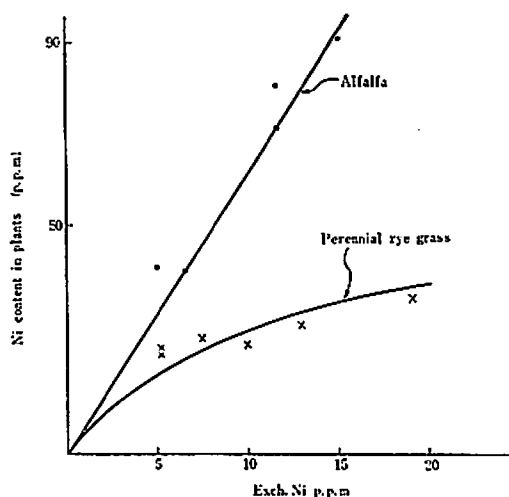
Fig. 3 Relation between exchangeable Ni in soils and Ni contents in plants
