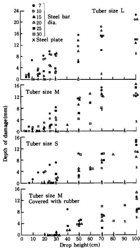
Fig. 8 Influence of impact surface, tuber size and drop height on depth damaged
