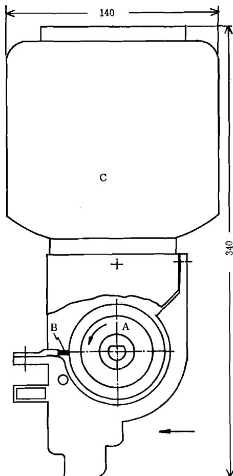
Fig. 2 Seed metering unit of rotor type planter
