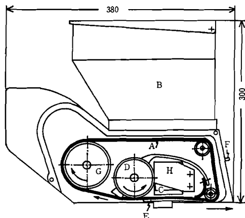
Fig. 1 Seed metering unit of belt type planter
