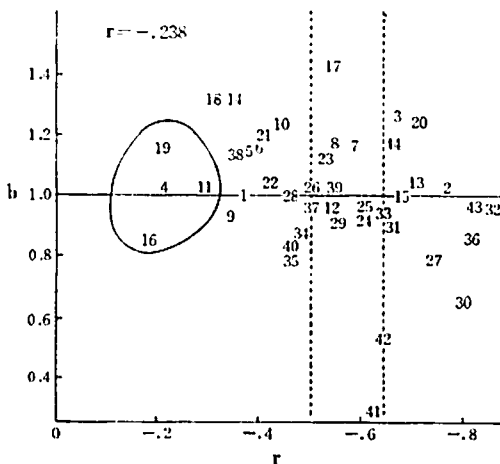
Fig. 7 A diagram showing relation between regression coefficients(b) of tuber yield and correlation(r), damage index of late blight and tuber yield (Broken lines show significant level at 1 and 5%)
