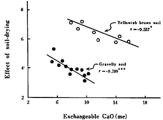
Fig 5 Relation between amount of exchangeable CaO and effect of soil-drying on the two converted soils at 3rd years after conversion (1972)
