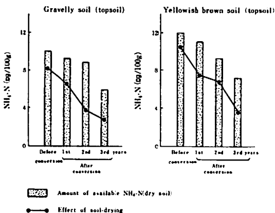
Fig 4 Change of available \text{NH}_4\text{-N} and effect of soil-drying on soil with the conversion of paddy field
