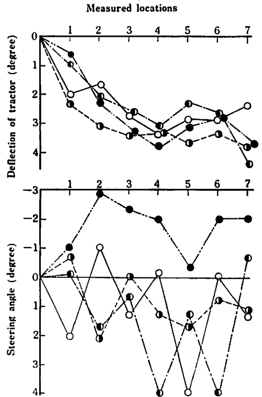
Fig. 8 Rotary plow
