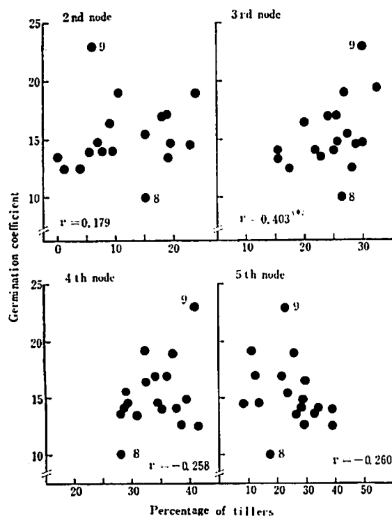
Fig. 3 Correlation between germinability at low temperature and percentage of tillers in each nodes at most active tillering stage (July, 18th, 1967)
