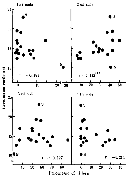
Fig. 2 Correlation between germinability at low temperature and percentage of tillers in each node at early tillering stage (July, 3rd, 1967)
