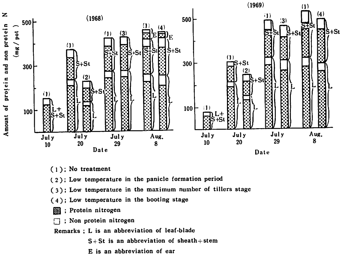
Fig. 6 Effect of low temperature on the composition of nitrogen uptake by rice plant
