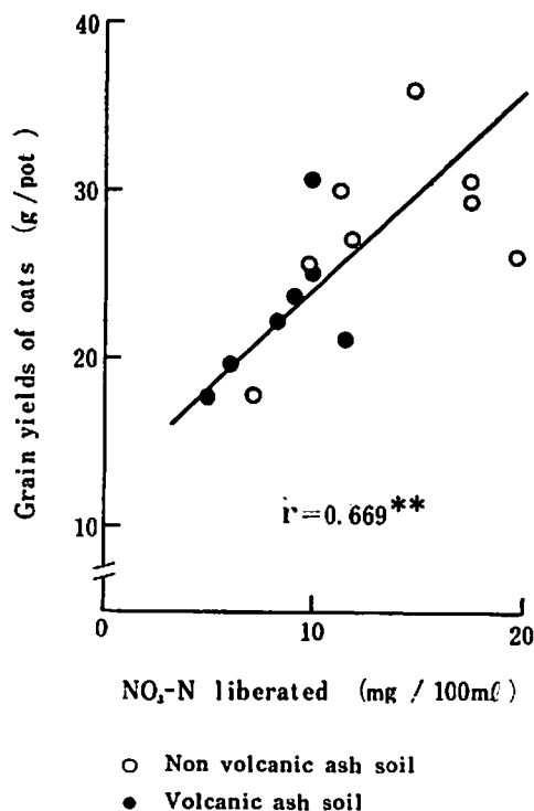
Fig. 3 Relation between \text{NO}_3\text{-N} in soils liberated on the leaching incubation and grain yields of oats
