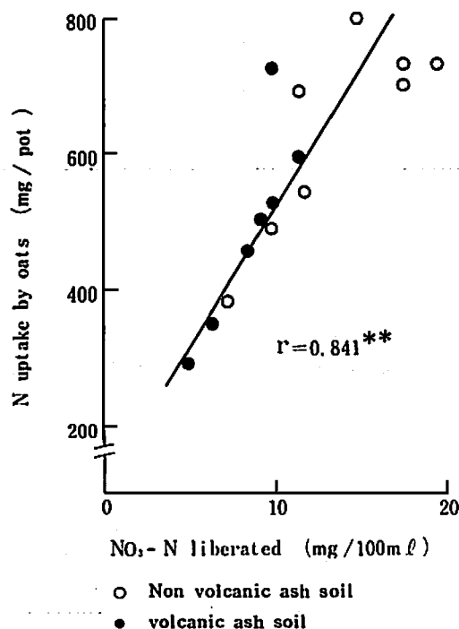
Fig. 1 Relation between \text{NO}_3\text{-N} in soils liberated on the leaching incubation and N uptake by oats
