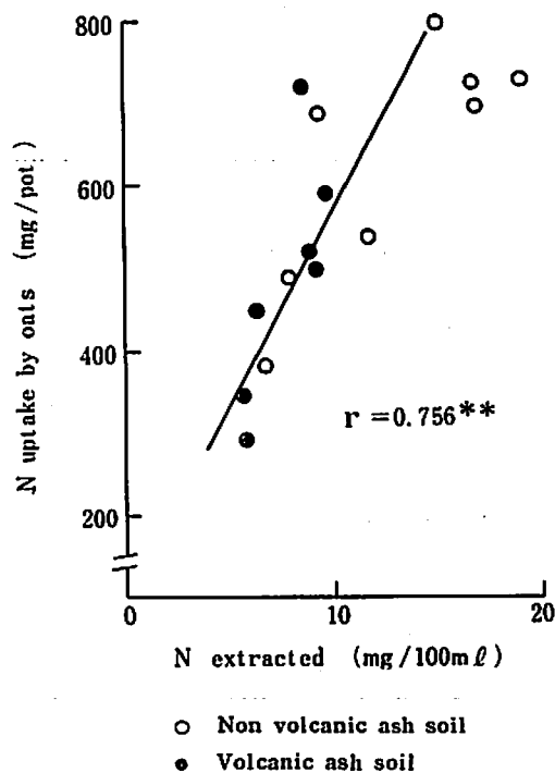
Fig. 2 Relation between N in soils extracted with hot water and N uptake by oats
