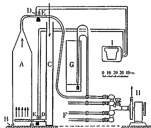
Fig. 1 Apparatus of chamber method
